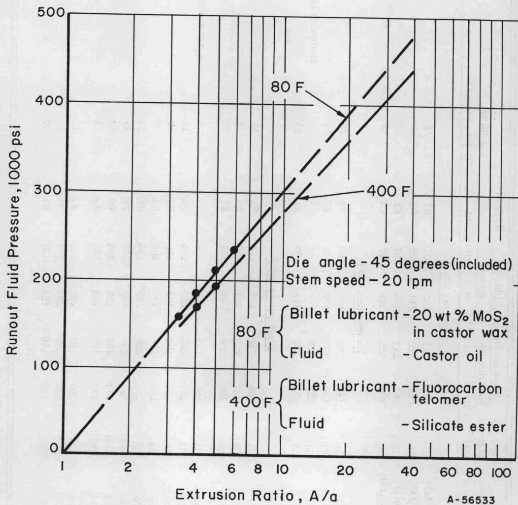
FIGURE 17. EFFECT OF EXTRUSION RATIO ON PRESSURES REQUIRED FOR HYDROSTATIC EXTRUSION OF AISI 4340 STEEL
